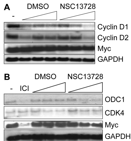
Fig. 7. The Northern blot suggests that compound NSC13728 inhibits Myc target gene transcription in avian and mammalian cells. CEF (A) or MCF7-35IM (B) were incubated with increasing amounts of media alone (-), 1 \mu\text{M} ICI 182,780, DMSO alone, or compound NSC13728. Total DMSO volumes were constant at all three dilutions alone and with compounds. Compound NSC13728 was used at 2.5, 5, and 10 \mu\text{M} .
