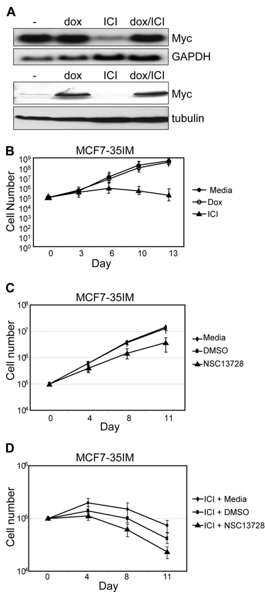
Fig. 6. Max homodimerization stabilizers are nontoxic to and complement growth inhibition by Myc depletion in MCF7-35IM. A, Northern blot (top two panels) and Western blot (bottom two panels) of MCF7-35IM in the presence of 1 \mu\text{g/ml} doxycycline or 1 \mu\text{M} ICI 182,780, where indicated. B to D, growth curves of MCF7-35IM in the presence of doxycycline or ICI 182,780 (B), compound NSC13728 (C), or NSC13728 plus ICI 182,780 (D). Cells were plated at 10^5 cells per well of 12-well tissue culture plates and were grown to \sim 80\% confluence. At the indicated time points, cells were trypsinized, counted, and replated to the initial concentrations. To calculate growth, the fold increase in cell number for each count was multiplied by the total number at the previous time point.
